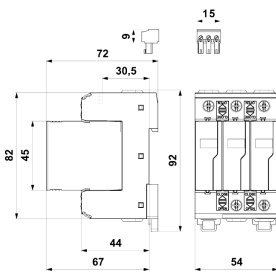
Dimension drawing
