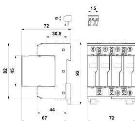
Dimension drawing
